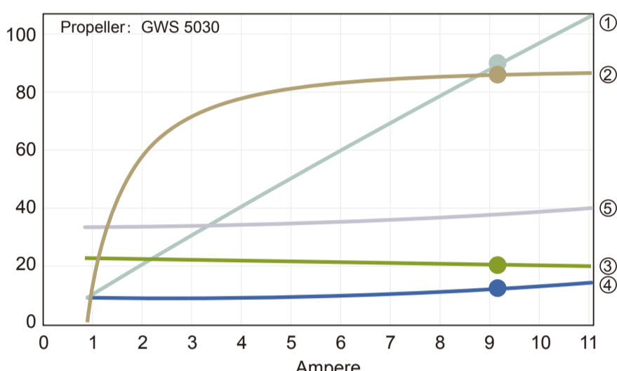
Motor Characteristics
